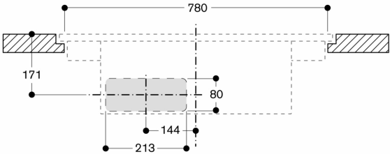
Front view - furniture cut-out for unducted recirculation; flush installation
