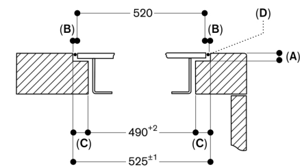
A: 6.5 +0.5 B: 2.5 C: 17.5 D: Fill with silicone measurements in mm
