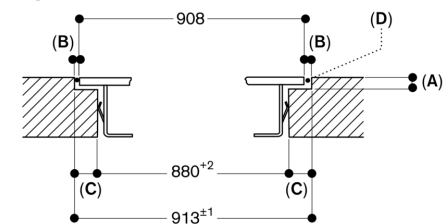
A: 6.5 +0.5 B: 2.5 C: 16.5 D: Fill with silicone measurements in mm
