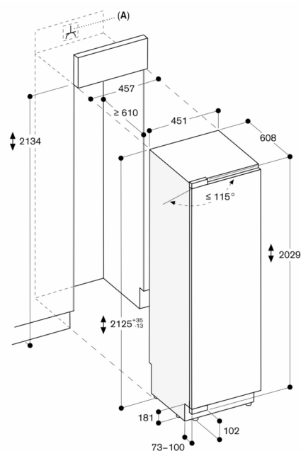
A: Socket Maximum door panel dimensions are based on a clearance of 3 mm
