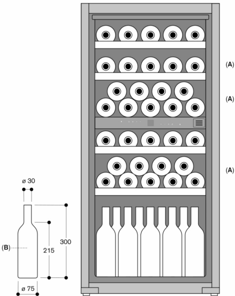
A: Suitable area for storage of magnum bottles in standard tray configuration B: 0.75 litres Measurements in mm
