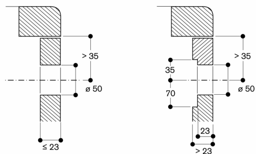
Installation of the control knob; surface mounting
